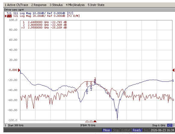
Wideband response (0-6GHz) Off state
