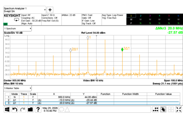
2 tones 50Wave 100Wpeak at 955MHz
