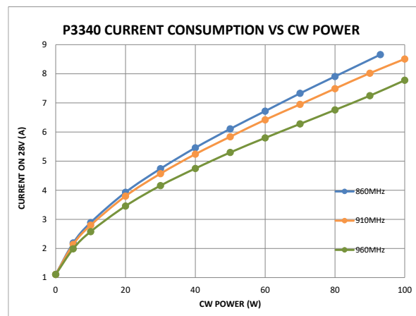
Current consumption on 28V vs CW power
