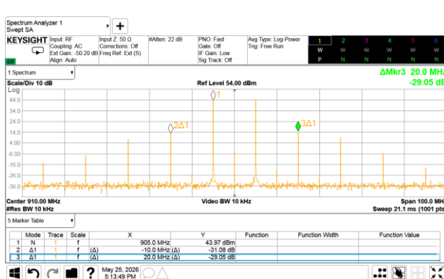
2 tones 50Wave 100Wpeak at 910MHz
