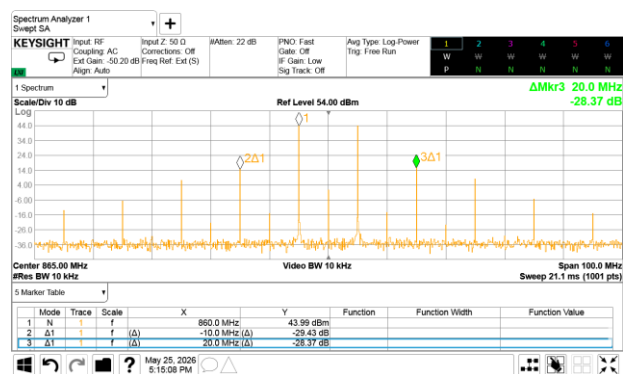
2 tones 50Wave 100Wpeak at 865MHz
