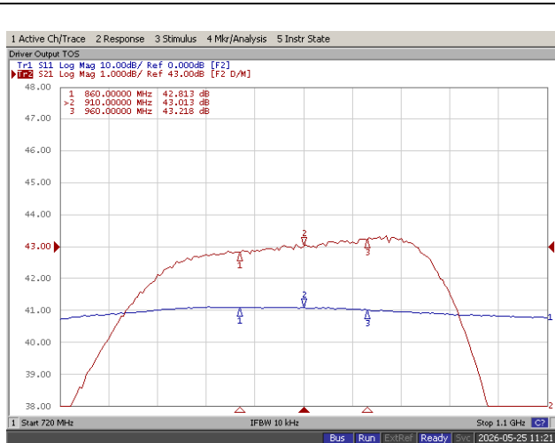
Gain / IRL vs frequency
