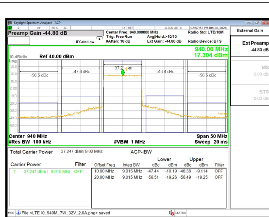
LTE10; 5Wave; 940MHz; 28V/1.8A
