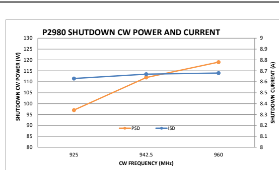
Shutdown current and CW power vs frequency
