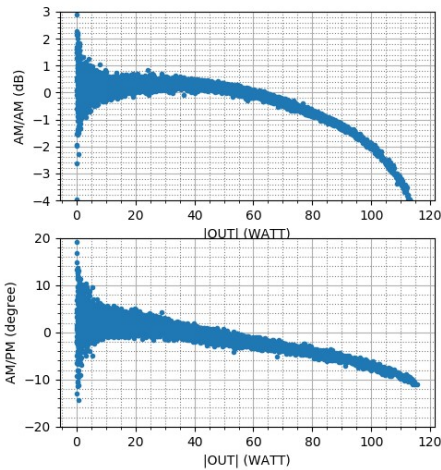
AMAM/AMPM ; LTE10; 28V
