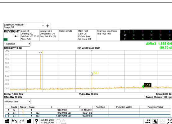
2nd and 3 rd Harmonics at 100W output
