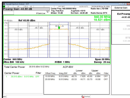
LTE10; 7Wave; 940MHz; 32V/2.0A
