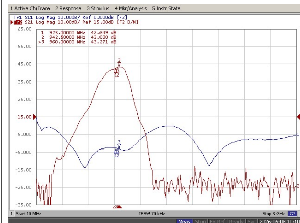
Wideband response (10-3000MHz)
