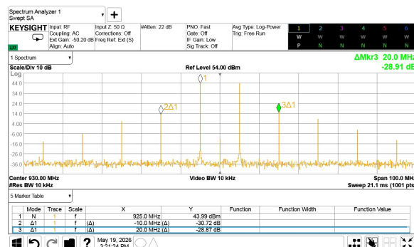
2 tones 47dBm ave / 50dBm peak at 925MHz
