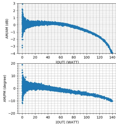
AMAM/AMPM ; LTE10; 32V
